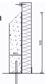
IP 50R 1500 x 100 x 500 mm
